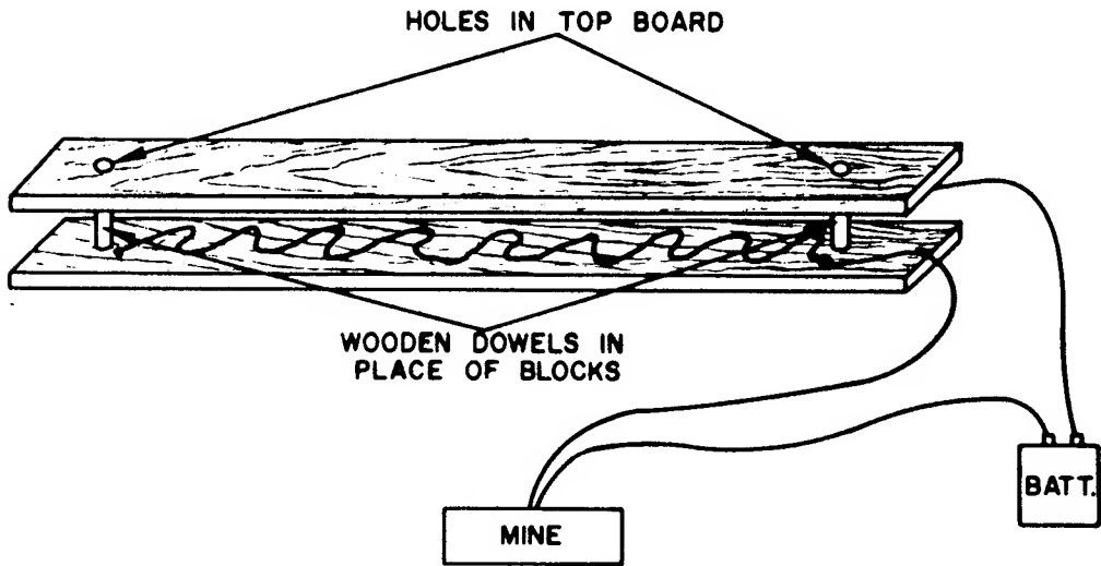
Figure 38. Pressure firing devices.
